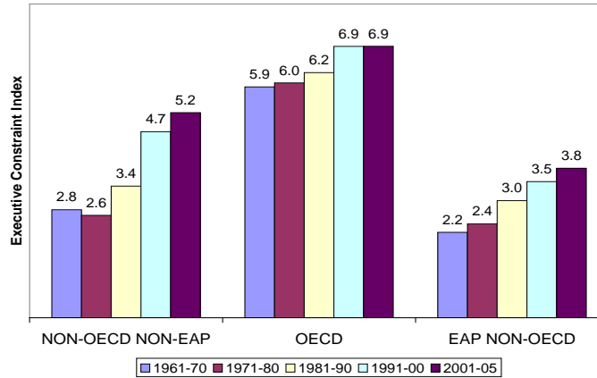
Figure 7: Institutional quality
