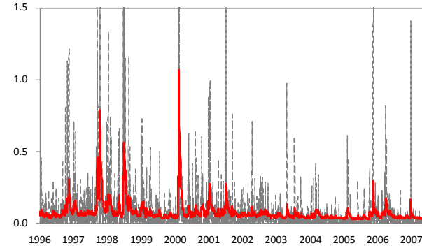
One-day-ahead prediction of the variance of \ln C
