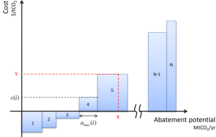
Figure 1: An expert-based MAC curve exhibits abatement options 1..N characterized by their maximum potential a_{max} and their marginal cost c , ranked from the least to the most expensive one. The classical interpretation, challenged in this paper, is that the optimal strategy for achieving abatement X is to implement all the activities cheaper than Y.
