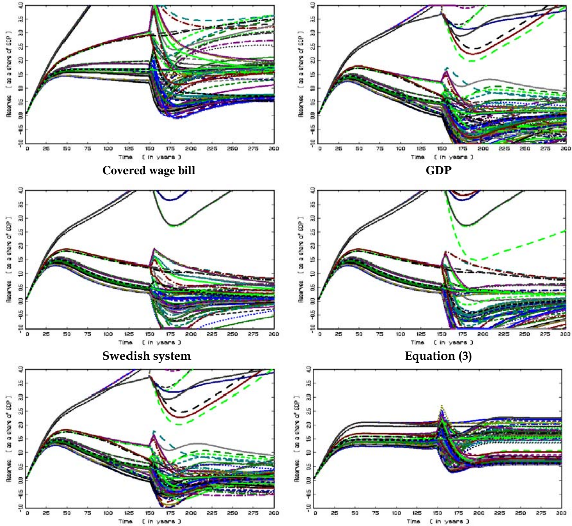
Figure 3: Dynamics of the Reserves/GDP Ratio When Annuity Does Not Include a Discount Rate
