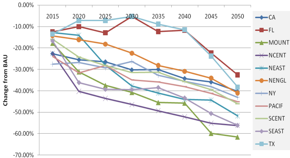
Figure 10. GHG Emissions Reductions by Region (Scenario TAAS).
