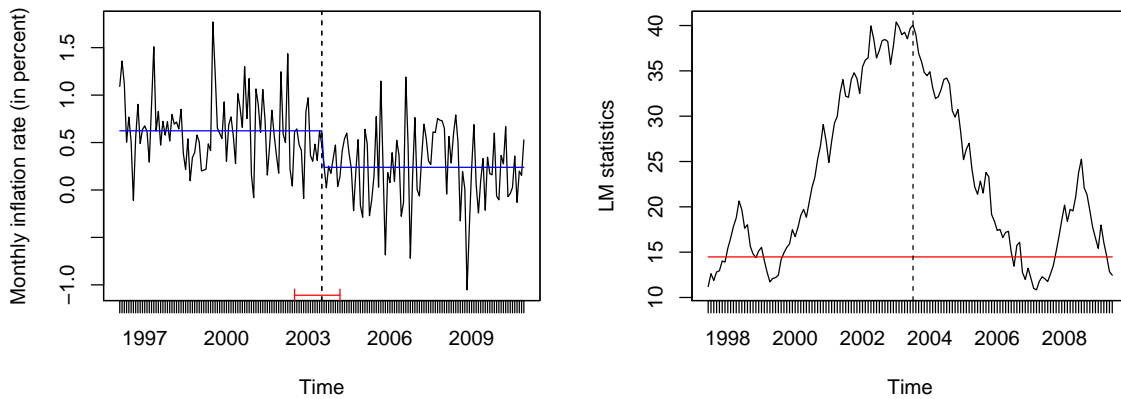
Figure 1: Inflation rate series for Slovenia with breakpoint estimate (Jul 2003), associated confidence interval, and fitted mean from generalized logistic distribution (left). Corresponding sup LM test (right) with sequence of LM statistics, critical value at 5% level (horizontal red line), and estimated breakpoint (vertical dashed line).
