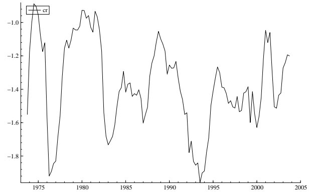
Figure 1. Australia and Canada. From top to bottom: earnings yield, earnings yield/government bond yield and cointegration relationship (nominal data). Left figures are for Australia, right figures for Canada.
