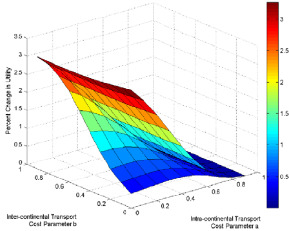
Fig. 2: Percent Change in 1A's Utility from an FTA Between Large (Top) or Small (Bottom) Economies
