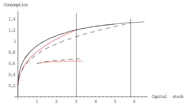
Figure 3 – Jointed phase diagram for the maximization problem (eq. 9) (the dashed dynamics represents the second scenario starting point).
