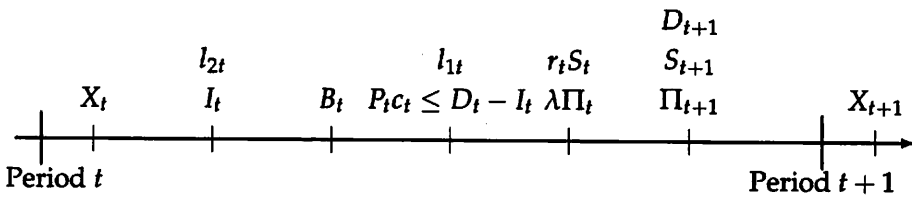
Figure 5 : The Sequence of Events with Cash-in-Advance Timing
