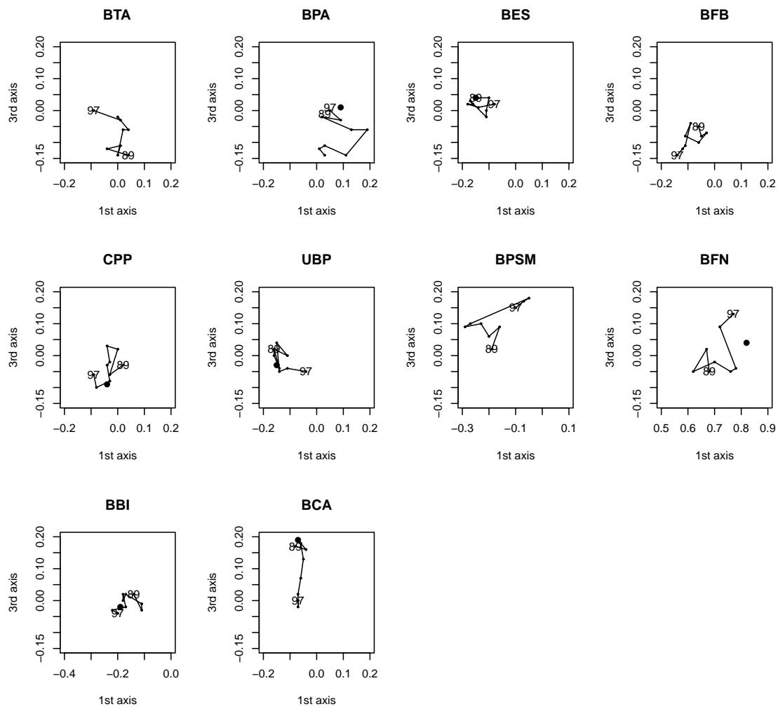
Figure 3: Trajectory of each bank around its compromise position (plane 1-3).
