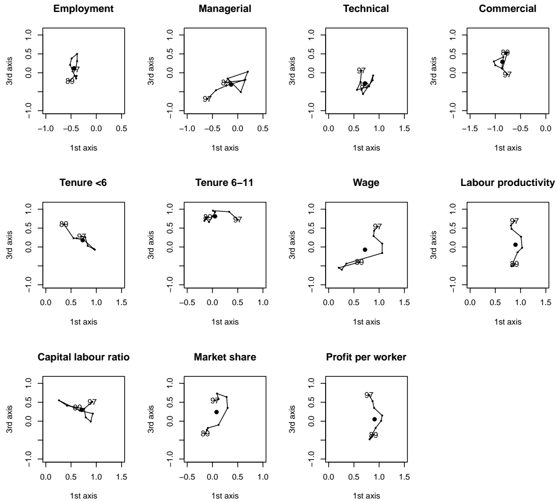
Figure 5: Trajectory of each variable around its compromise position (plane 1-3).
