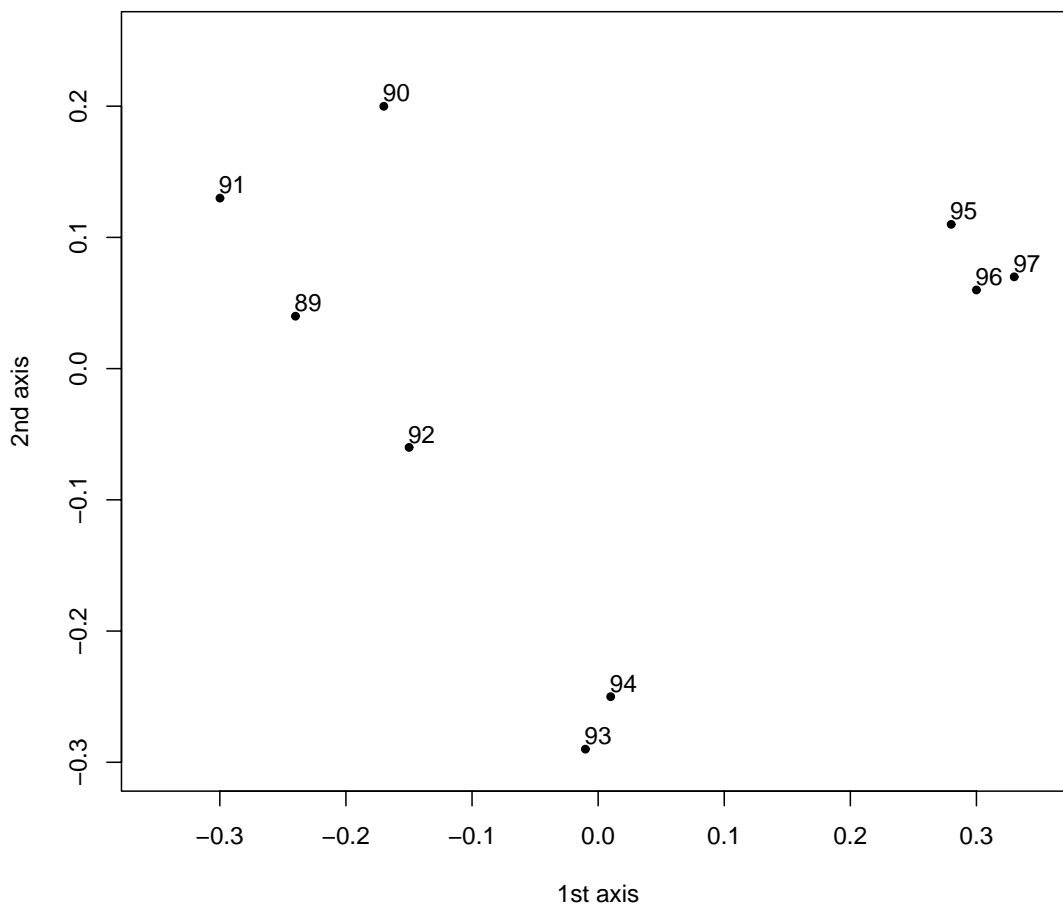
Figure 1: Euclidean image of the interstructure (Statis).
