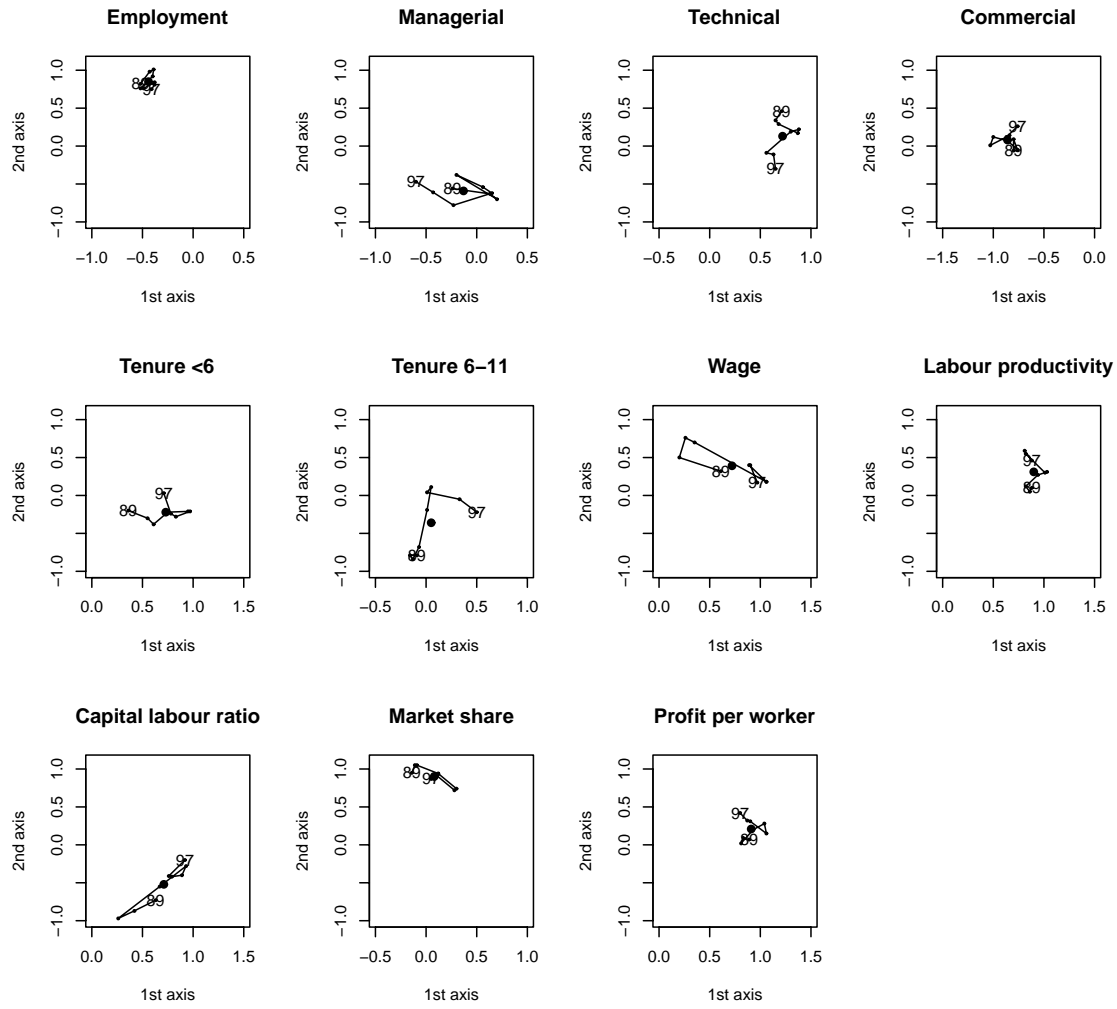
Figure 4: Trajectory of each variable around its compromise position (plane 1-2).
