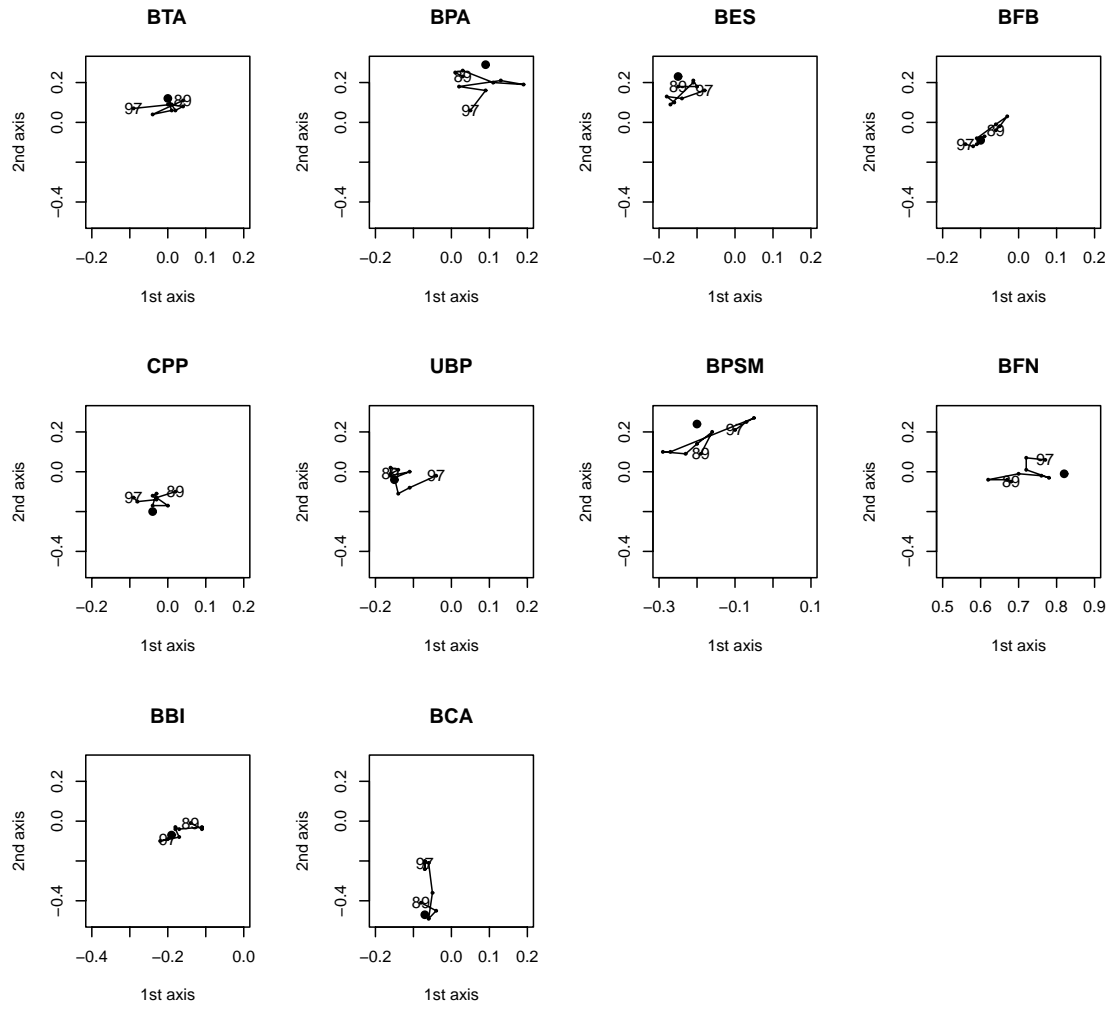
Figure 2: Trajectory of each bank around its compromise position (plane 1-2).
