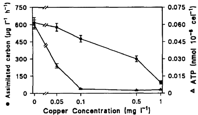
Fig. 1. Photosynthetic rate as assimilated carbon ( \mu\text{g l}^{-1} \text{h}^{-1} ) and intracellular ATP content ( \text{nmol} \times 10^{-6} \text{ cell}^{-1} ) of Phaeodactylum tricornutum cells exposed to different copper concentrations ( \text{mg l}^{-1} ),
