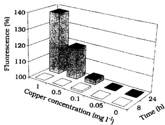
Fig. 3. Chlorophyll a fluorescence after copper exposure in Phaeodactylum tricornutum cells. Data on chlorophyll a fluorescence are expressed as the percentage of the fluorescence of control cells, according to the equation of Reader et al. (1993). Results are the means of three replicates.
