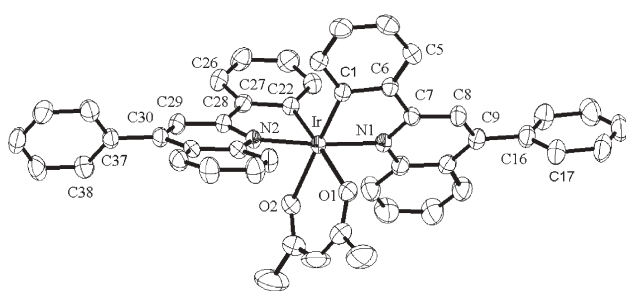
Fig. 1 ORTEP drawing of \text{Ir}(\text{DPQ})_2(\text{acac}) with thermal ellipsoids representing a 50% probability level. Hydrogen atoms have been omitted for clarity.
