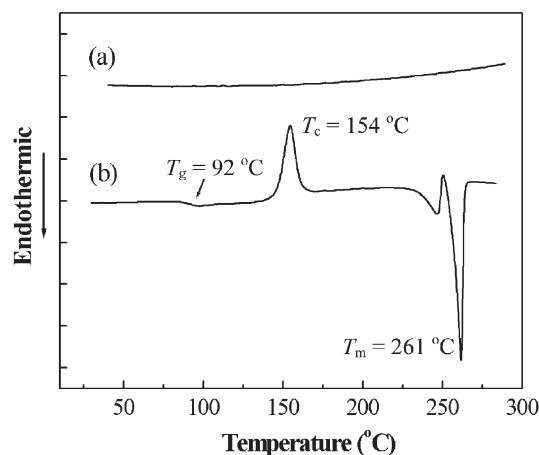
Fig. 2 Differential scanning calorimetry (DSC) data for (a) \text{Ir}(\text{DPQ})_2(\text{acac}) and (b) \text{Ir}(\text{FPQ})_2(\text{acac}) (heating rate: 20^\circ\text{C min}^{-1} ) under nitrogen.
