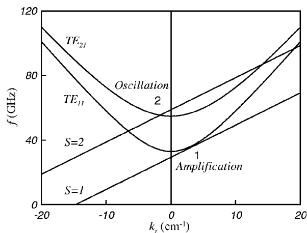
FIG. 1. \omega-k_z diagrams of the waveguide modes and the beam wave synchronism lines for a TE_{11} mode, 34-GHz gyro-TWT, operating at the fundamental cyclotron harmonic.
