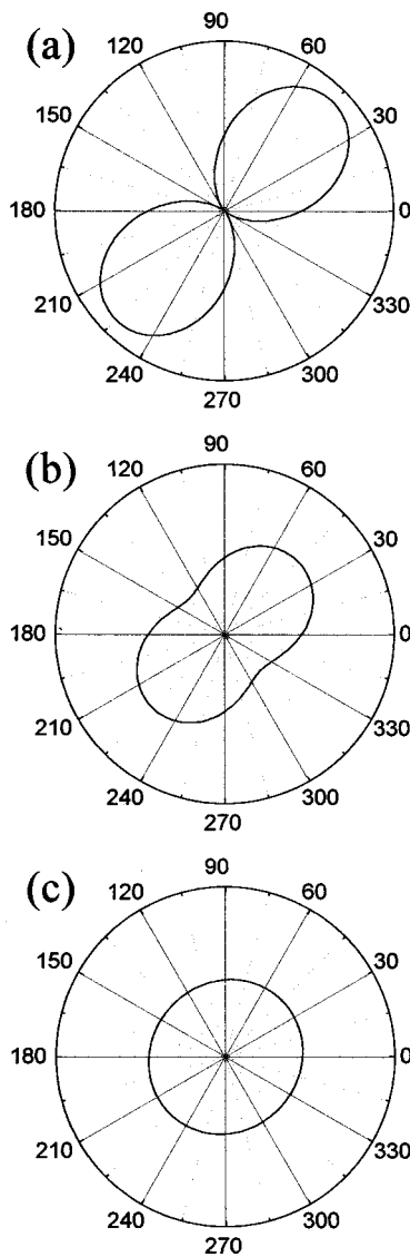
FIG. 6. Measured polarization states of the 2.45 GHz output wave emerging from the converter with (a) an unsqueezed converting section, (b) and under-squeezed converting section, and (c) an optimally squeezed converting section.
