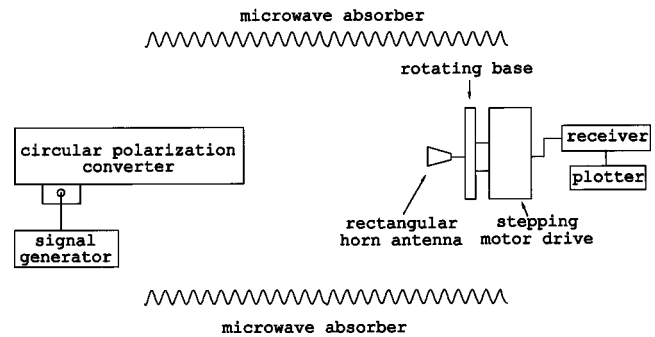
FIG. 4. The test setup for polarization measurement of the output wave from the converter.
