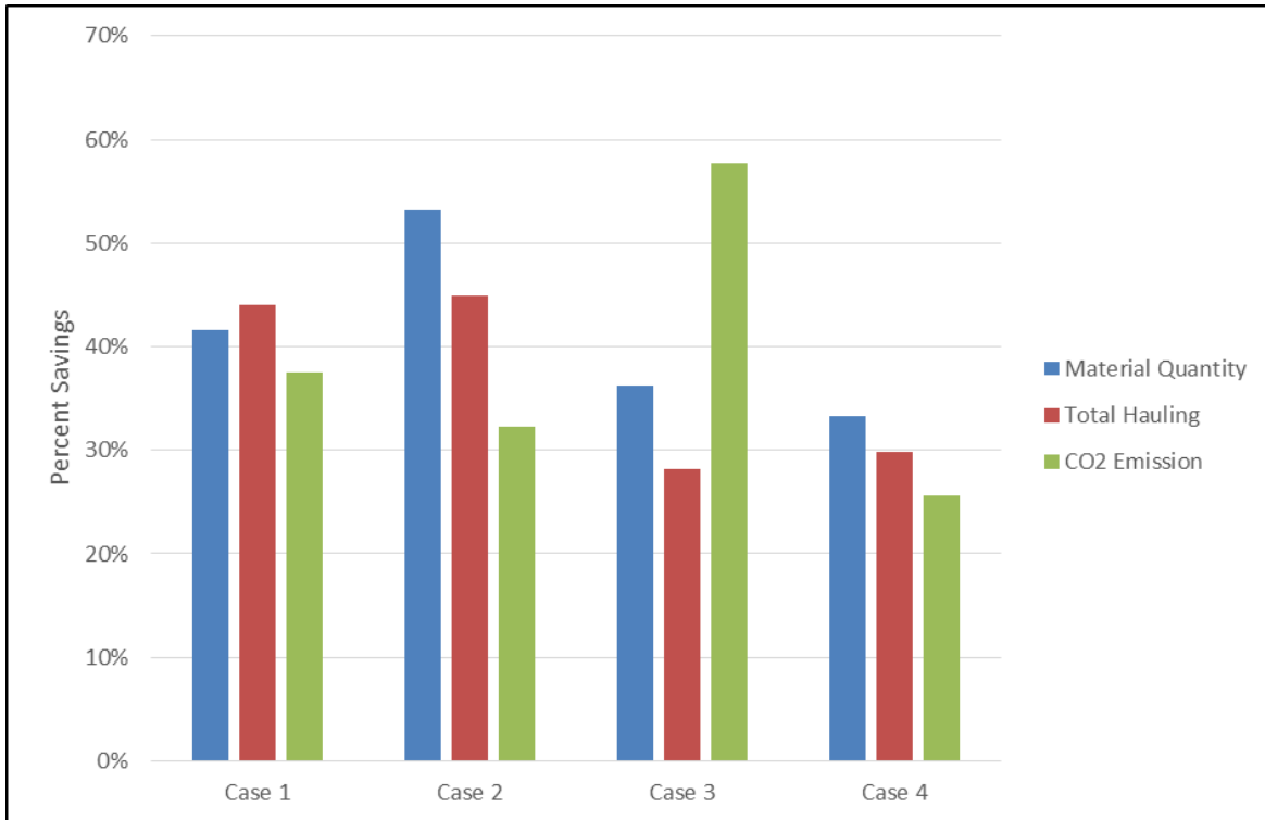
Figure 6: Percentage saving achieved by using Neoloy Geocells in different projects (case)
