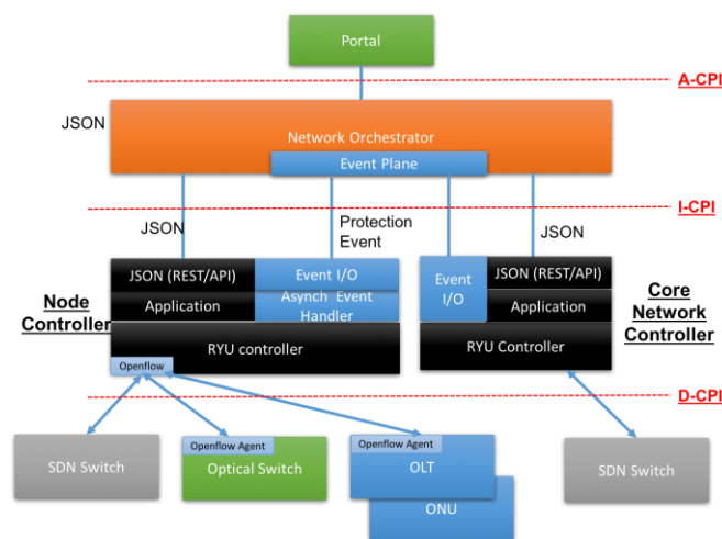
Fig. 3. Architecture of the overall SDN control plane.
