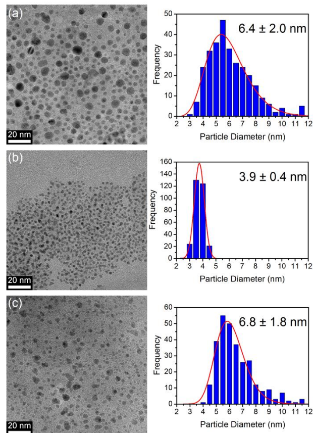
Fig. 1: Left, TEM images of the (a) parent solution, (b) supernatant and (c) pellet. Right, histograms of the NC size with curves fitted to the data using a lognormal model in the case of (a) and (c) and a Gaussian model in the case of (b).
