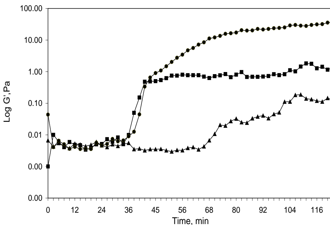
Figure 3.10. Influence of acidification by 30 g L -1 GDL at 32°C on the storage modulus, G', of bovine (●), asinine (■) or equine (▲) milk. The coefficient of variation was <5% of the reported value for each data point.
