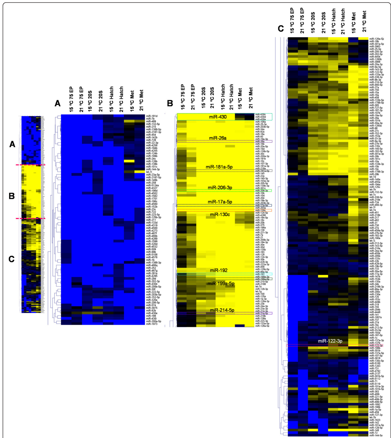
Figure 2 Heatmap of conserved miRNAs obtained by SOLiD sequencing during Senegalese sole early development. The complete heatmap (normalised to the number of trimmed reads, log 2 transformed, Euclidean distance, complete linkage) has 320 rows (miRNAs) and 8 columns that correspond to 4 developmental stages (75Ep, 20S, hatching and metamorphosis) and two embryonic temperatures (15 and 21°C). For visualisation purposes, the heatmap was split in 3 panels: A) miRNAs with a low number of reads throughout development, B) miRNAs consistently expressed at high levels at all stages, and C) miRNAs with variable expression through development. Yellow and blue indicate higher and lower expression levels, respectively. miRNAs frequently referred to in the main text are highlighted in larger font.
