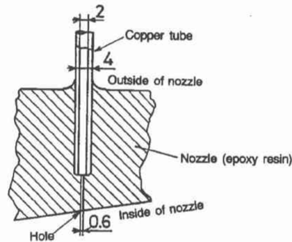
Figure 2(B). Cross section near a pressure tap.
