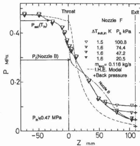
Figure 6. Pressure profiles of the nozzle with a small convergent angle.
