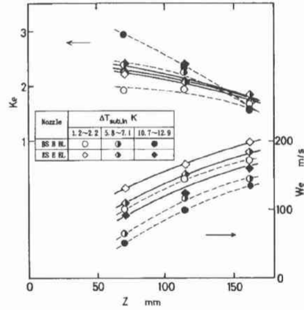
Figure 10. Velocity and liquid phase velocity.
