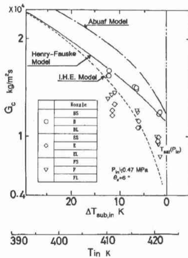
Figure 11. Critical flow rate.
