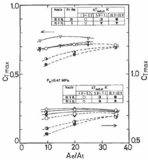
Figure 15. Maximum thrust coefficient for the conventional and improved nozzles.
