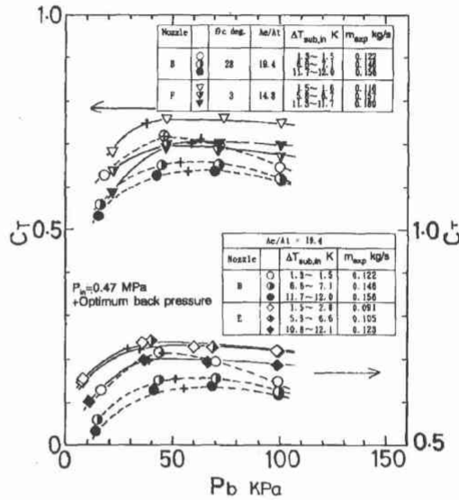
Figure 14. Thrust coefficient for the conventional and improved nozzles.
