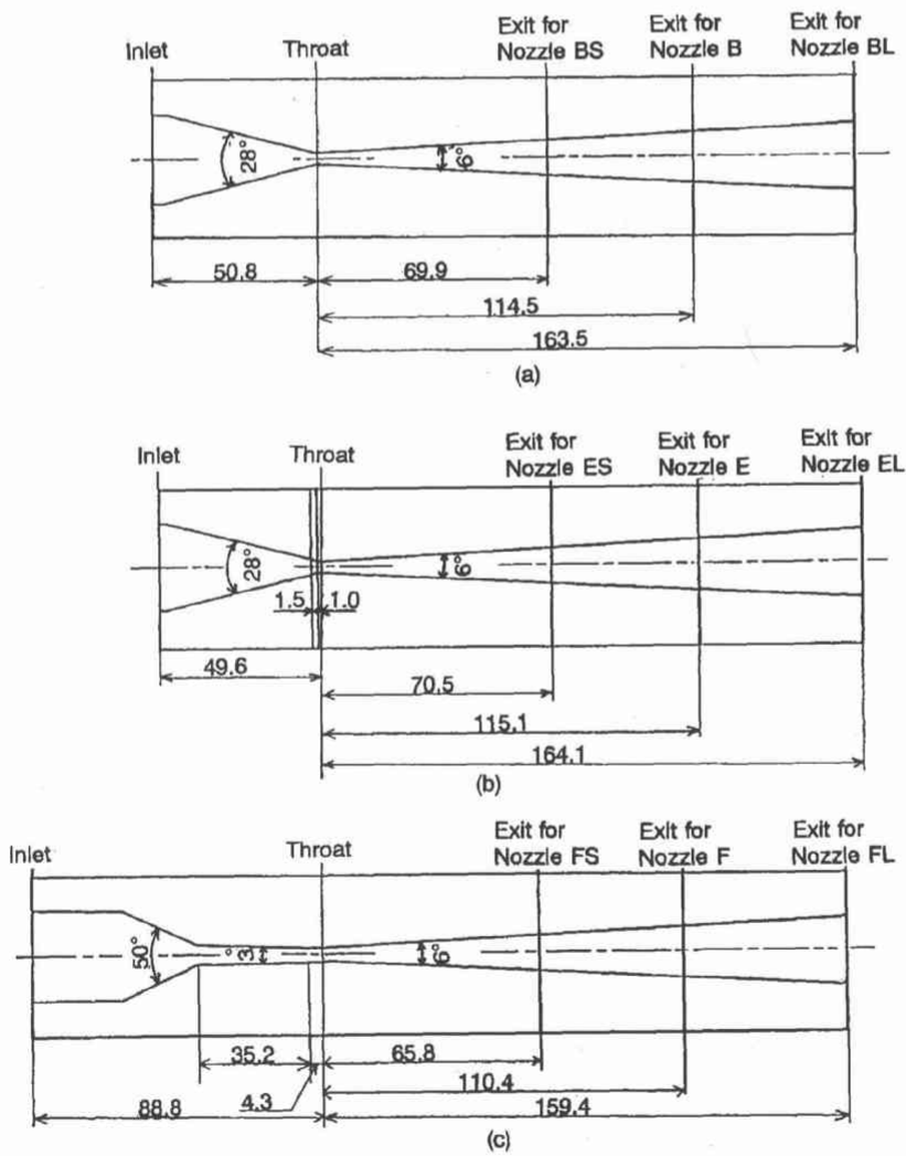
Figure 2(A). Cross sections of the nozzles.
