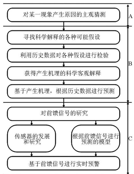
图 1 地震预报和天气预报的一般研究路线 Fig 1 Common research route of earthquake prediction and weather forecast
