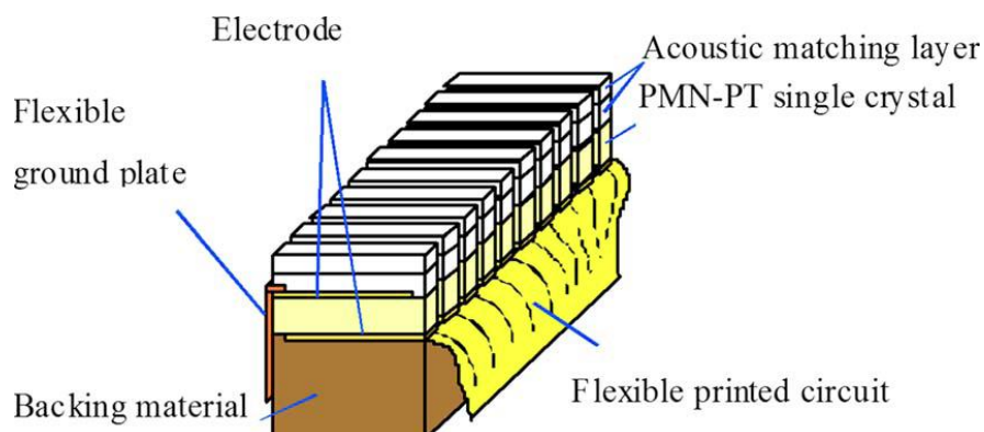
Figure 16. Schematic diagram of the PMN-PT phased array (with permission from [24]).
