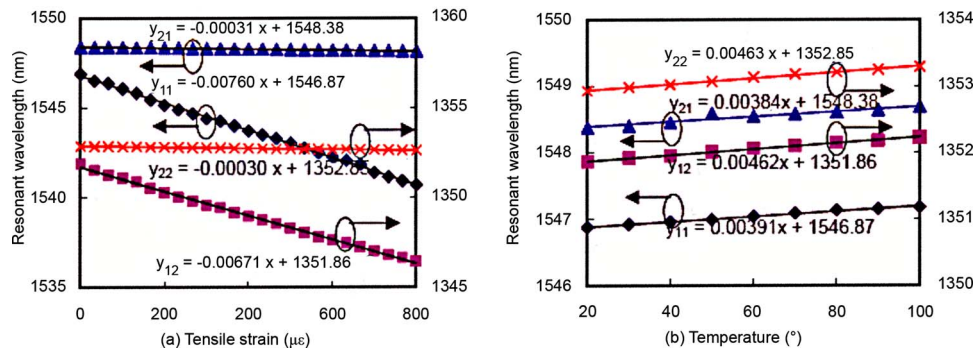
Fig. 5. (Color online) Resonant wavelength of LPFG 1 and LPFG 2 via (a) the tensile strain and (b) the temperature. \blacklozenge , Dip 11 of LPFG 1 ; \blacksquare , Dip 12 of LPFG 1 ; \blacktriangle , Dip 21 of LPFG 2 ; \times , Dip 22 of LPFG 2 .
