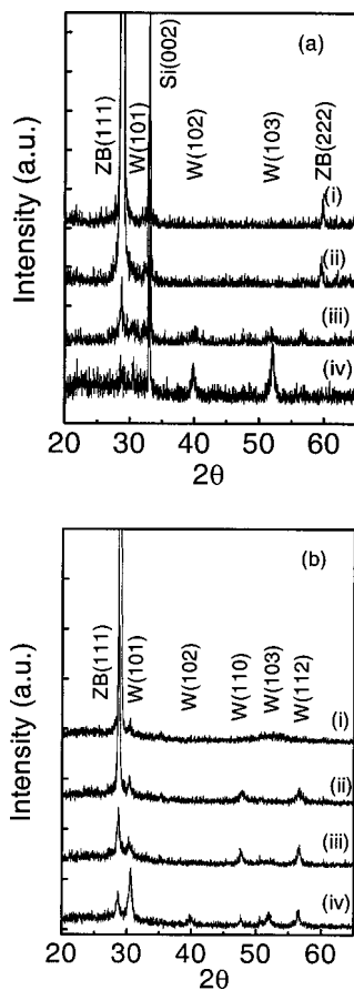
FIG. 8. XRD patterns of the ZnS:Mn films grown on (a) (001)Si with deposition temperature of (i) 150 °C, (ii) 250 °C, (iii) 350 °C, and (iv) 450 °C; on (b) ITO-coated glass with deposition temperatures of (i) 150 °C, (ii) 250 °C, (iii) 350 °C, and (iv) 450 °C.
