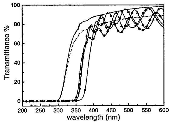
FIG. 5. Transmittance of ZnS:Mn films deposited on ITO-coated glass at 150 °C (—■—), 250 °C (—●—), 350 °C (—▲—), and 450 °C (—◆—). The transmittance spectra for ITO-coated glass before (—) and after (—●—) annealing at 500 mTorr of oxygen for 30 min are also shown for comparison.
