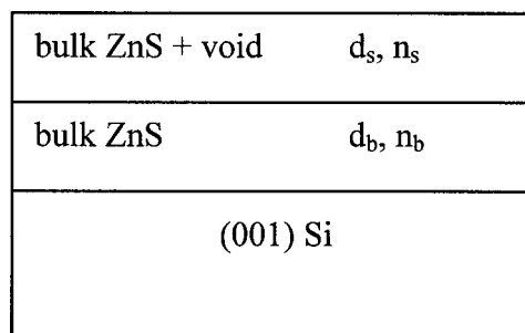
FIG. 2. Schematic picture of the double layer Sellmeier (DLS) model.
