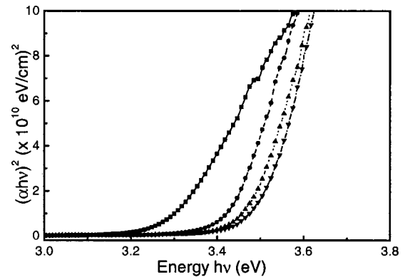
FIG. 6. Profiles of (\alpha h\nu)^2 against h\nu for ZnS:Mn films deposited at 150 °C (—■—), 250 °C (—●—), 350 °C (—▲—), and 450 °C (—◆—).
