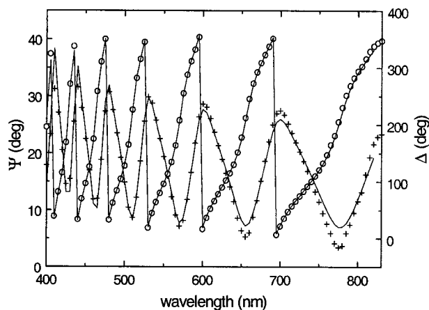
FIG. 1. Spectra of the ellipsometric parameters \psi and \Delta as functions of wavelength from SE experiments of ZnS:Mn film deposited at 350^\circ\text{C} . The (+) and (O) are the measured \psi and \Delta values, respectively, while the solid lines are model fitting.
