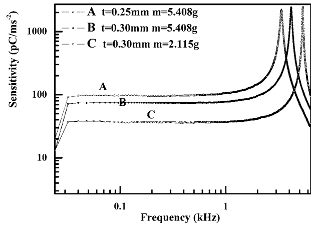
FIG. 3. The sensitivity of the cymbal-based accelerometers as a function of frequency.
