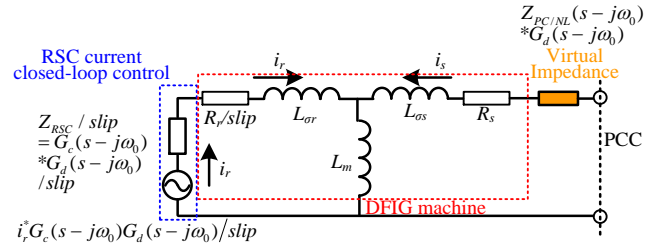
Fig. 7. Impedance modeling of RSC and DFIG machine with the introduction of virtual impedance in the DFIG stator branch through stator current feedforward control
