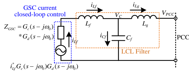
Fig. 2. Impedance modeling of Grid Side Converter (GSC) and LCL filter
