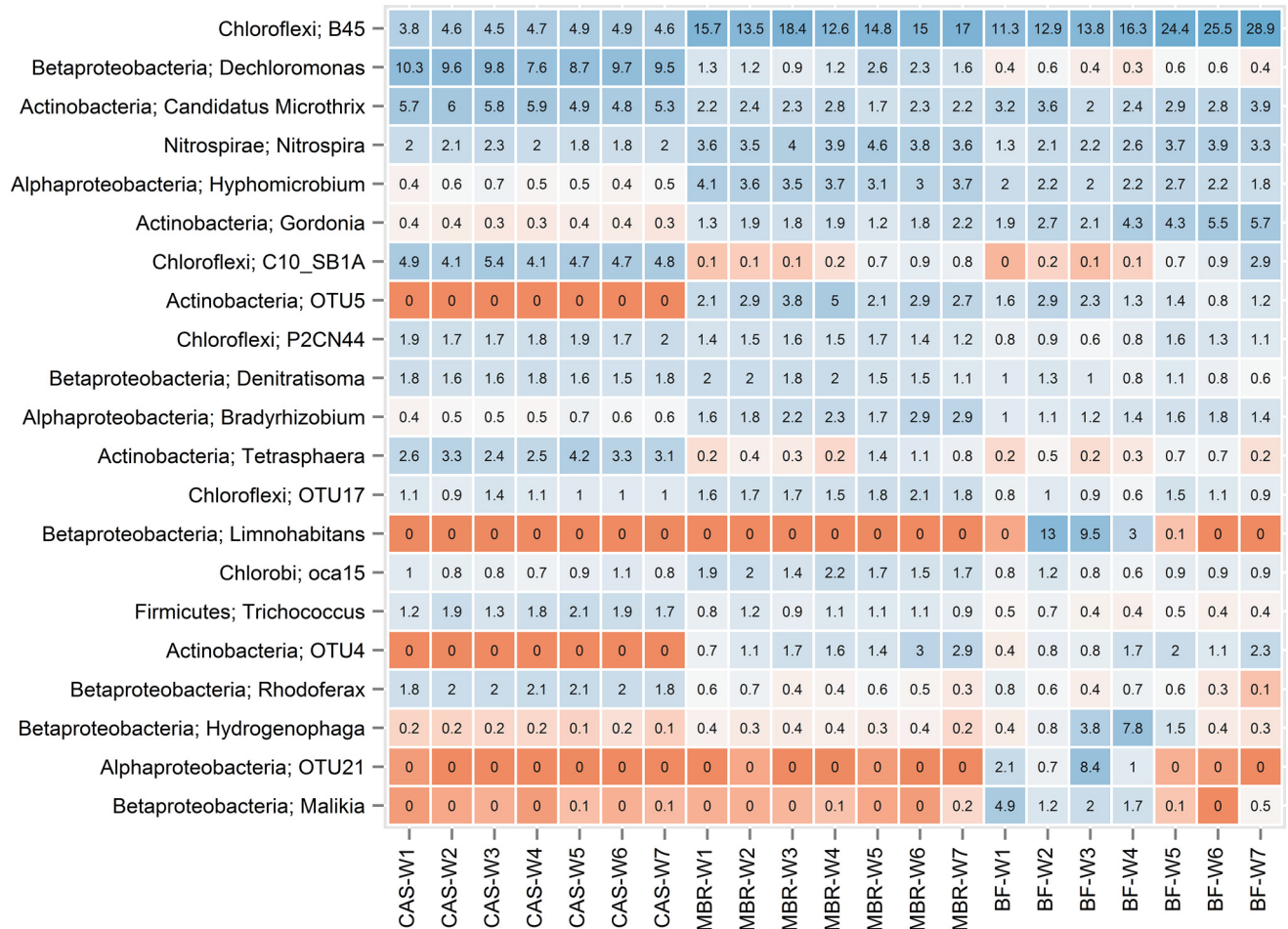
Fig 3. Heatmap showing the microbial composition represented as the 10 most abundant genera of CAS bulk sludge samples (CAS), MBR bulk sludge samples (MBR) and biofilm samples (BF), combined yielding 21 genera. The OTU number is given if it was not classified to the genus level with the MiDAS taxonomy. The data is visualised as a table with underlying colours showing changes and numbers showing the relative read abundances. W1-7 indicate the sampling time (in weeks).
