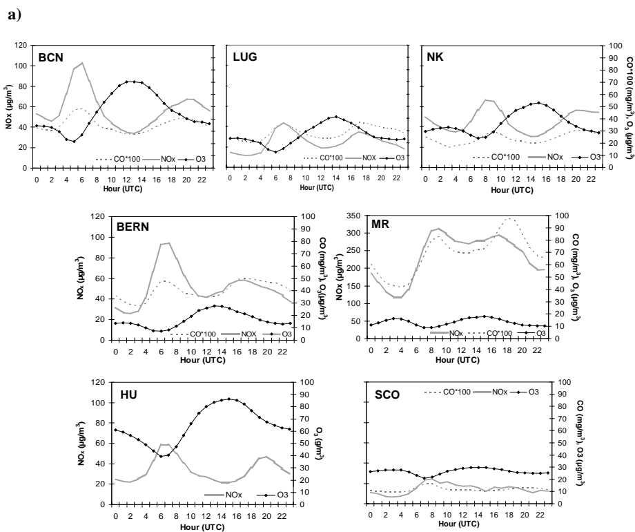
Fig. 2a. Daily cycle of: gaseous pollutants concentrations ( \text{CO} , \text{NO}_x and \text{O}_3 ) levels for each monitoring site.
