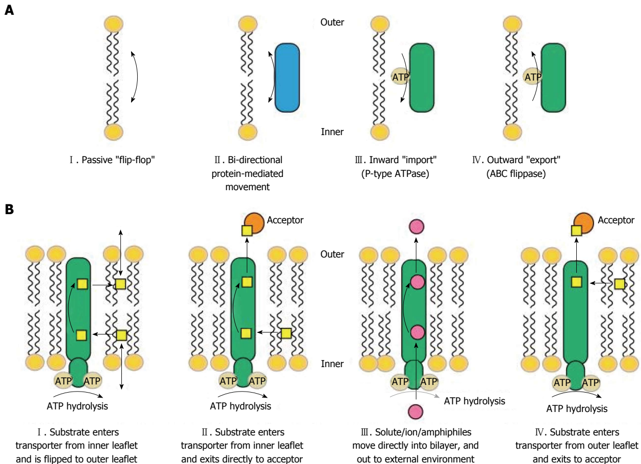
Figure 1 The models presented are from Tarning et al. [16] . A: Lipids can move across the membrane bilayer by multiple mechanisms. Four mechanisms are proposed here: (1) membrane lipids passively diffuse or "flip-flop" from one leaflet of the bilayer to another; (2) bi-directional movement of lipids from one membrane leaflet to another is enhanced by proteins present in the membrane bilayer; (3) P-type ATPases mediate the movement of specific lipids (phospholipids) from the outer leaflet of the membrane bilayer; and (4) ABC transporters/flippases mediate the "outward" movement of specific lipids (phospholipids/cholesterol) from the inner leaflet to the outer leaflet of the membrane bilayer; B: Mechanisms of substrate recognition and transport by ABC transport proteins: (1) substrates enter the transporter from the inner leaflet and are flipped to the outer leaflet where they can exit the membrane bilayer; (2) as in (1) but the substrate exits the transporter directly to an exogenous acceptor; (3) solute/ions/amphiphiles move directly into the bilayer, through the transporter protein and out to the external environment; and (4) substrates enter the transporter from the outer leaflet and exits to an acceptor molecule.
