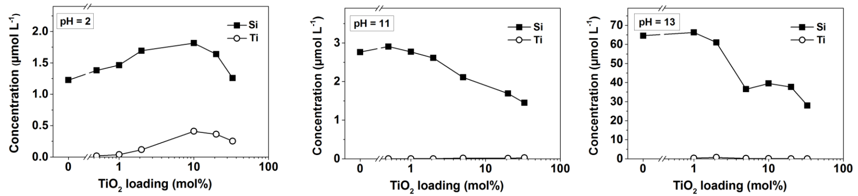
Fig. 6. Silicon and titanium concentration in the leached solutions at pH 2, 11 and 13, as measured by ICP-OES analysis.
