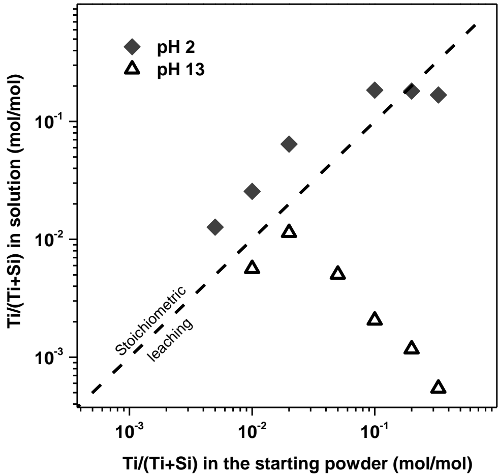
Fig. 7. Ti molar fraction in the leached solutions at pH 2 and 13 as a function of the Ti molar fraction in the starting powder. The dashed line indicates stoichiometric leaching, i.e. the dissolved material has the same composition of the starting powder.
