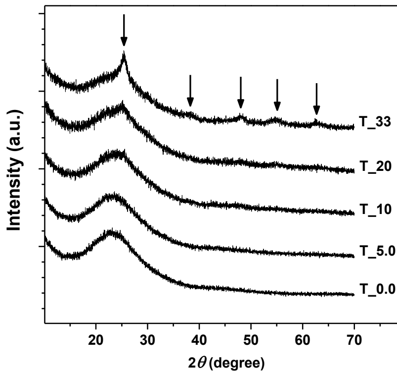
Fig. 1. XRD patterns of the TiO 2 -silica powders. The arrows indicates the peaks typical of the anatase phase, visible in the sample T_33.
