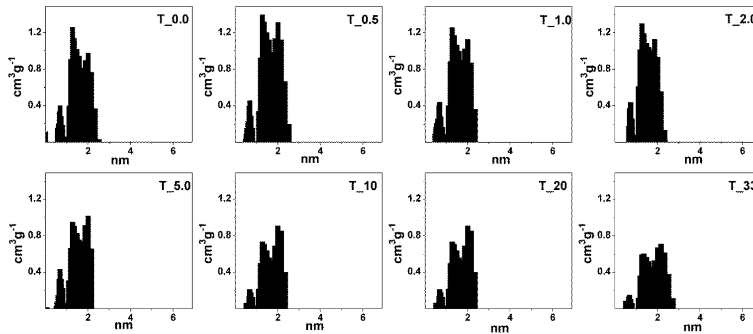
Fig. 5. DFT pore size distribution of the eight materials presented in this study.
