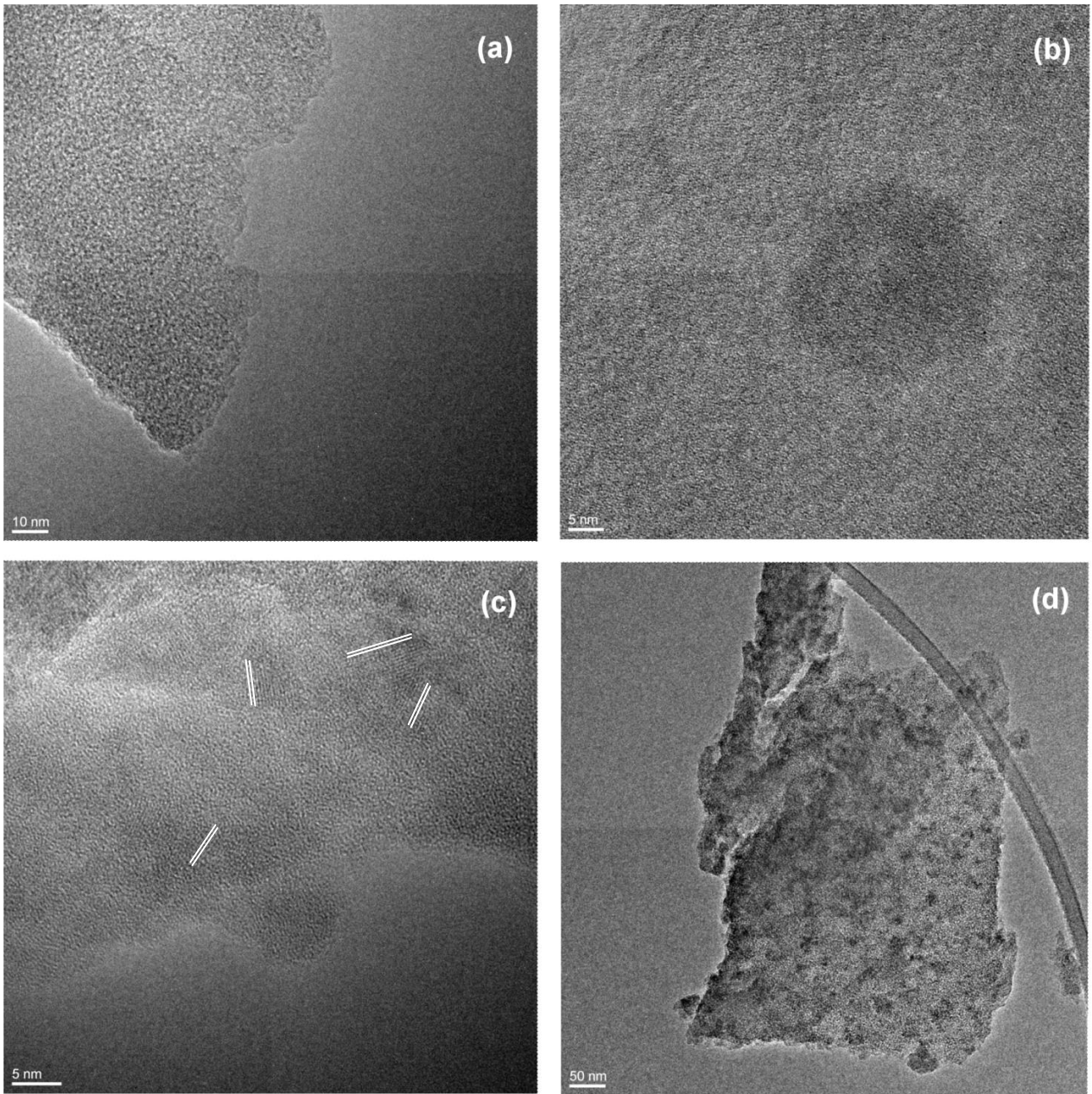
Fig. 2. TEM pictures of the sample T_0.0 (a), T_5.0 (b), T_10 (c), and T_20 (d). White lines in section (c) stress fringe patterns of the anatase \text{TiO}_2 nanocrystals. A detailed description of the micrographs is given in the text (section 3.2).
