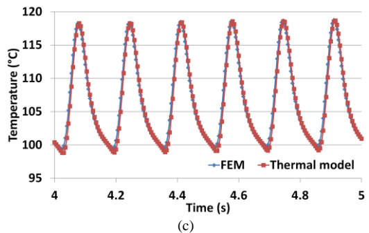
Fig. 16. Junction temperatures from simulated simplified thermal model and FEM simulation at different boundary conditions: h_{tc}=20000 \text{W/m}^2\cdot\text{K} (a), T_C=120^\circ\text{C} (b), P_{loss}=100 W (c).
