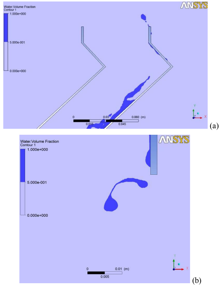
Figure 19. (a) Water volume fraction for VL2-Q4 case.
