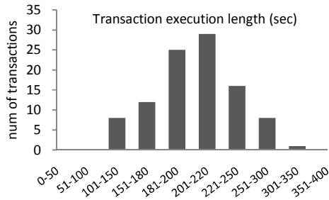
Figure 7. Distribution of transactions' lengths
