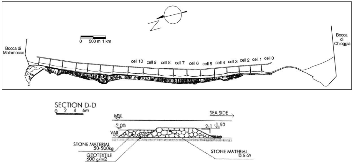
Fig. 9. Plan view of Lido of Pellestrina and LCS section.
