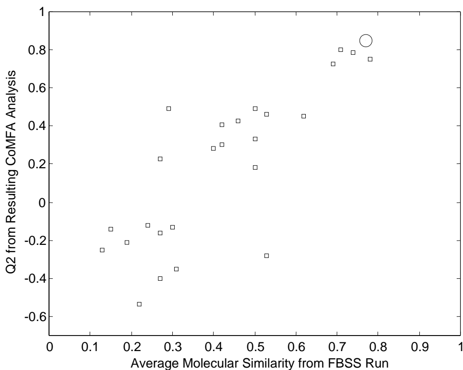
Figure 2. Plot of the average FBSS molecular similarity against the square of the cross-validated correlation coefficient, q^2 , for the steroid dataset. The circle point represents the results obtained with the manual alignments.
