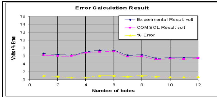
Figure 10: The error between COMSOL and experimental result
