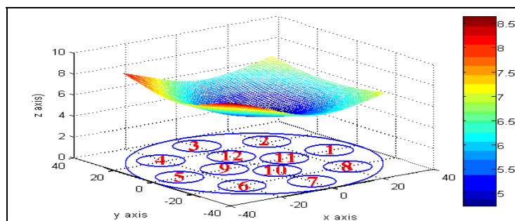
Figure 9: Result from COMSOL (same as the result from Configuration 1 section 4.1)
