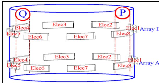
Figure 11: Arrangement of electrode array on the pipe
