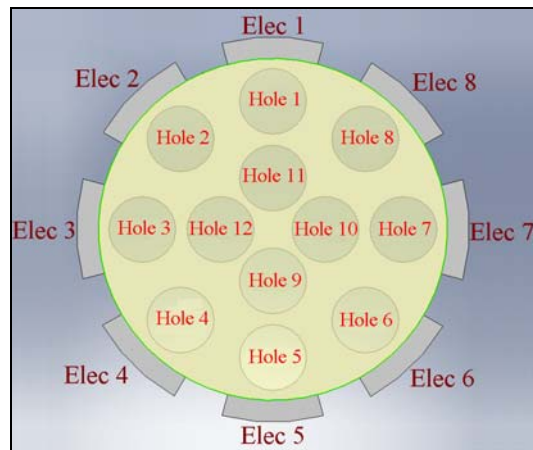
Figure 6: A 12 holes associated with different electrode
