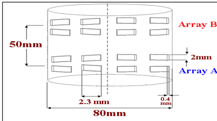
Figure 2: Arrangement of electrode array on the pipe
