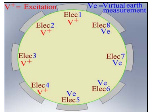
Figure 3: Array A electrode configuration
