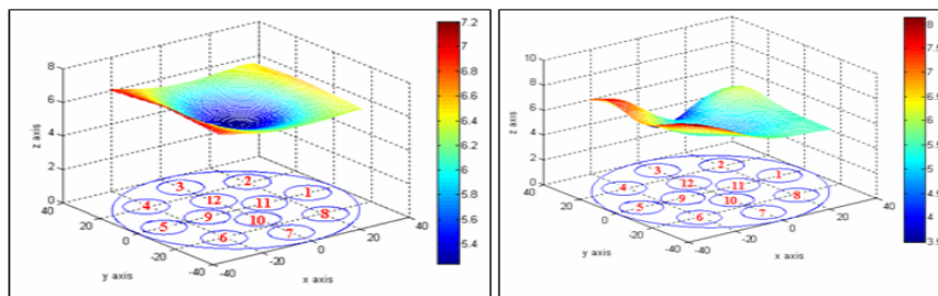
(a) Config-1 (b) Config-2 Figure 7: Sensitivity distributions
