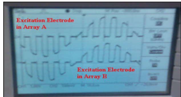
Figure 5: Excitation signals for excitation electrode in Array A & B
