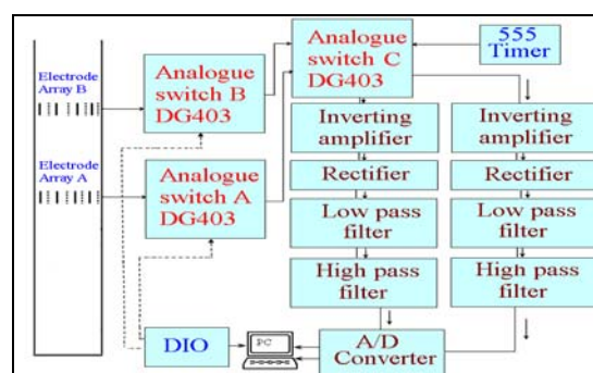
Figure 1: Schematic diagram of the data acquisition and control system.
