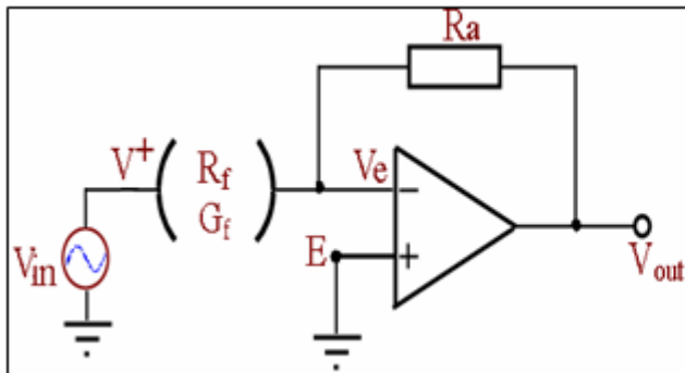
Figure 4: Fluid conductance circuit
