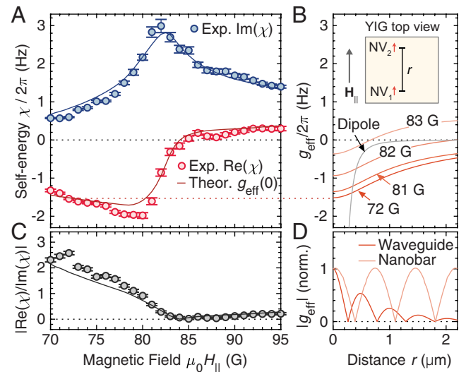
Fig. 4. Magnon-mediated coupling determined from magnon-induced self-energy. (A) Magnon-induced NV center self-energy \chi as a function of the magnetic field H_{\parallel} . The red (blue) markers represent the experimentally determined real (imaginary) part of \chi . The red (blue) curves show the theoretical predictions of g_{\text{eff}}(r=0) = \text{Re}(\chi) and \text{Im}(\chi) , respectively. (B) Calculated NV–NV distance r dependence of the effective NV–NV coupling strength g_{\text{eff}}(r) mediated by magnons at multiple fields H_{\parallel} . Two NV centers are placed at the same distance h_{\text{NV}} = 400 nm from the YIG surface and displaced in the direction of \mathbf{H}_{\parallel} as shown in the Top illustration. The dipole-dipole interaction strength g_{\text{dip}}(r) is shown with a gray curve as a reference. (C) Ratio of the real and imaginary parts of \chi as the magnetic field is swept through the MSSW resonance, indicating how the ratio of NV–NV coupling to dissipation varies with the NV frequency. Markers and the gray curve are experimental and theoretical results, respectively. (D) Calculated g_{\text{eff}} as a function of r in different geometries of YIG, an infinitely long waveguide and a nanobar. Two curves are calculated for the identical long conditions as in ref. 17. The vertical axis is normalized by g_{\text{eff}}(r=0) .
