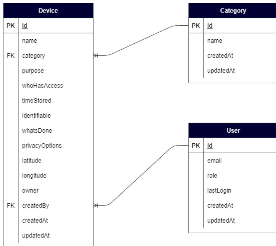
Fig. 14: Entity relationship diagram of database.
