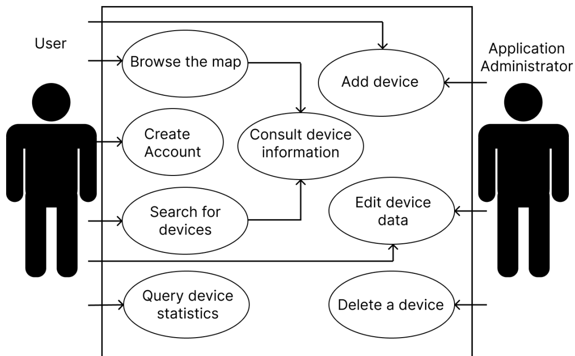
Fig. 9: Use cases diagram.
