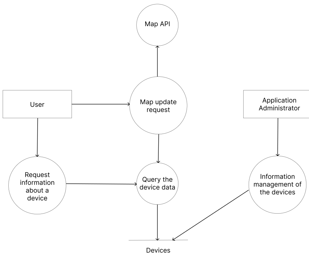
Fig. 7: Data flow diagram.
