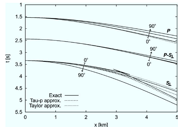
FIG. 7. Traveltimes for reflections from the bottom of the second HTI layer for P, S_{\perp} , and P- S_{\perp} converted waves. Traveltimes are computed for constant azimuthal phase angles of 0^{\circ} , 45^{\circ} , and 90^{\circ} . Solid line: exact curves; long dashes: \tau - p approximations; short dashes: Taylor-series approximations (along symmetry axis only).
