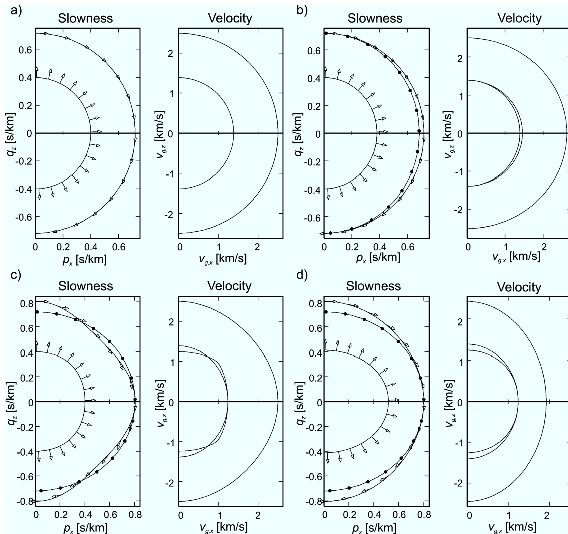
FIG. 1. Vertical slices of the slowness surfaces (left side) and wave surfaces (right side) for the second layer in four models. The particle motion for each wavenumber is indicated by vectors on the slowness surfaces. (a) Isotropic model, (b) transversely isotropic with a vertical symmetry axis (VTI), (c) vertically aligned fluid-filled fractures, (d) vertically aligned gas-filled fractures. The fracture density is 0.1, the aspect ratio is 0.001, and the normal to fracture plane is in the offset direction x . The anisotropic models display rotational symmetry around, respectively, the vertical (b) and horizontal axis [(c) and (d)].
