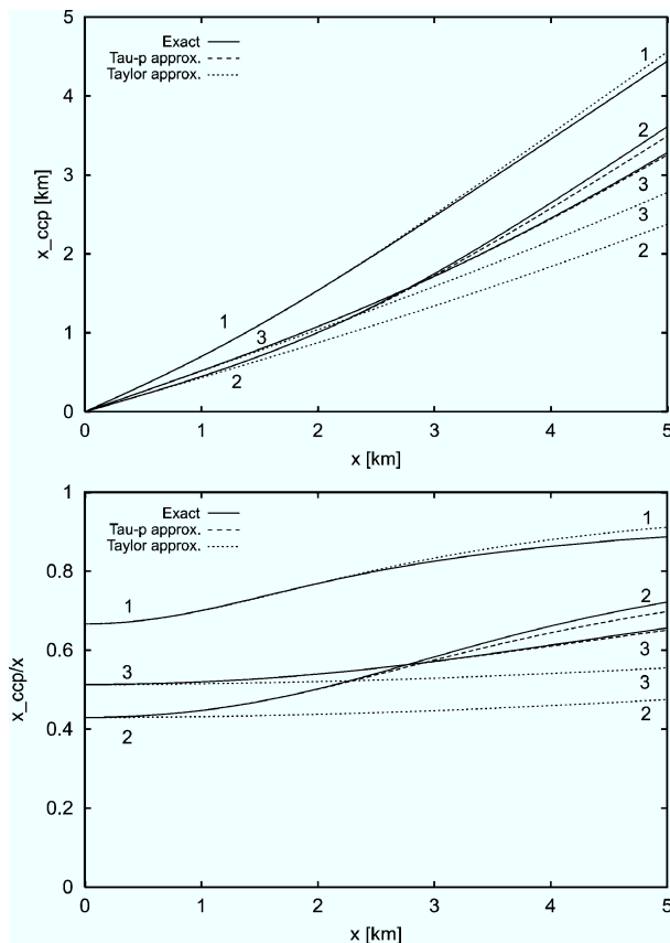
FIG. 6. Estimations of the common conversion points x_{ccp} of P- S_{\perp} converted waves for the three-layer VTI model. Upper part: conversion point distance from the source as a function of emergence offset. Lower part: ratio x_{ccp}/x . Numbers correspond to layer indices. Solid line: exact curves; long dashes: \tau - p approximations; short dashes: Taylor-series approximations.
