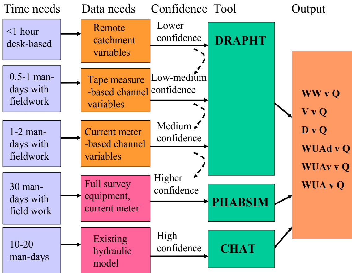
Figure 5.1 RAPHTSA flow chart
