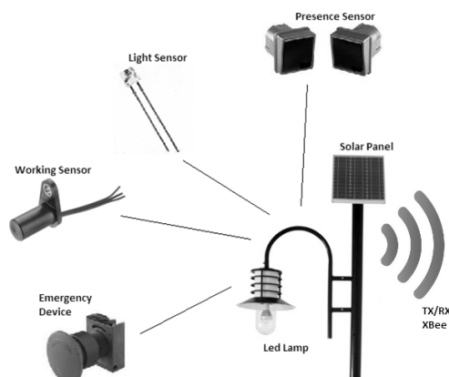
Figure 1. Scheme of the lamppost with sensors.
