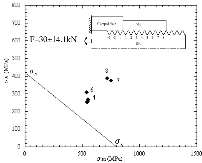
Figure 11. Endurance limit diagram for \alpha=\alpha_{small}
