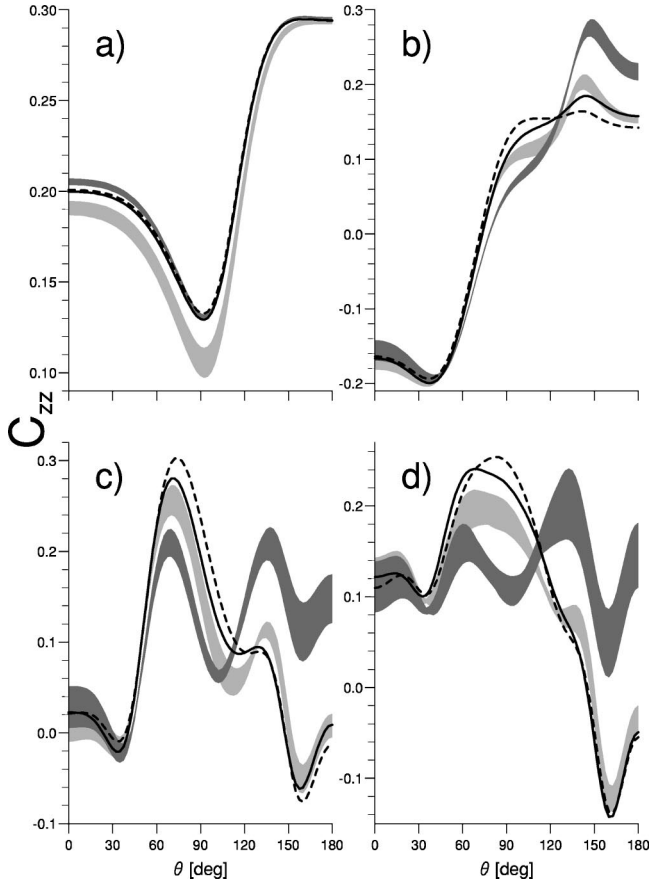
FIG. 14. The spin correlation coefficient C_{zz} for elastic Nd scattering. Curves and the sequence of energies as in Fig. 1.
