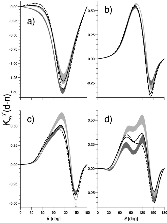
FIG. 8. The spin transfer coefficient K_{yy}^{y'} for elastic Nd scattering. Curves and the sequence of energies as in Fig. 1. pd data at 135 MeV from Ref. [22].
