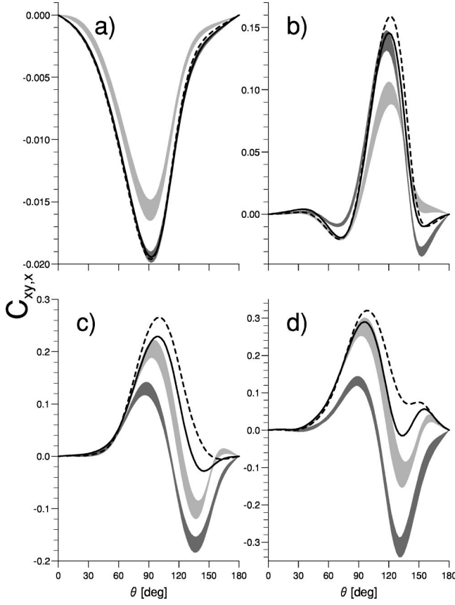
FIG. 12. The spin correlation coefficient C_{xy,x} for elastic Nd scattering. Curves and the sequence of energies as in Fig. 1.
