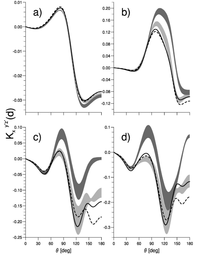
FIG. 11. The spin transfer coefficient K_x^{y'z'} for elastic Nd scattering. Curves and the sequence of energies as in Fig. 1.
