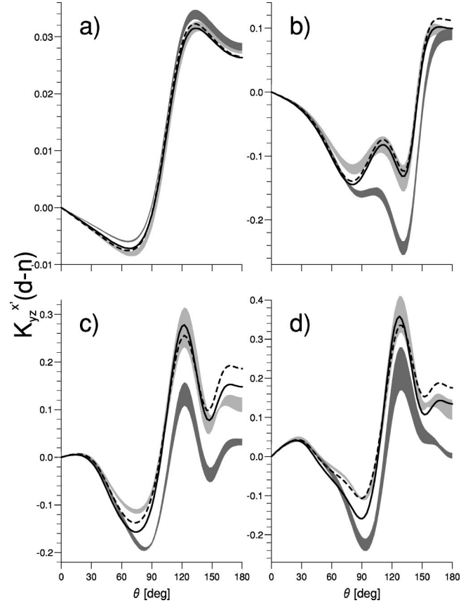
FIG. 7. The spin transfer coefficient K_{yz}^{x'} for elastic Nd scattering. Curves and the sequence of energies as in Fig. 1.
