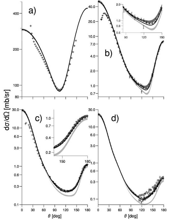
FIG. 1. The differential cross section in elastic Nd scattering at 3 (a), 65 (b), 135 (c), and 190 MeV (d). Two bands are shown in each subfigure, the light shaded one contains NN force predictions, the darker shaded one the NN force predictions+TM 3NF. The solid curves are the AV18+URBANA IX predictions. The dashed curves are the CD Bonn+TM' predictions. Data at 3 MeV from Ref. [60] ( pd ), at 65 MeV from Ref. [61] ( pd crosses), and Ref. [62] ( nd circles), at 135 MeV from Refs. [22] ( pd crosses), [23] ( pd circles), and at 190 MeV from [63] ( pd crosses 181 MeV, circles 216.5 MeV). In some cases error bars are not visible on the scale of the figure.
