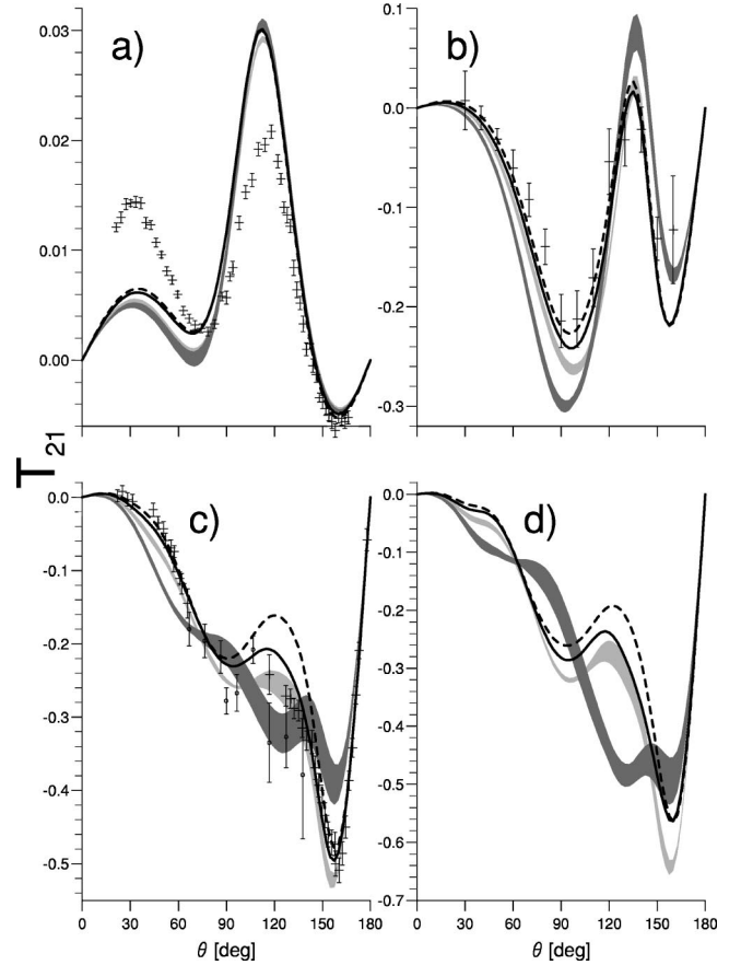
FIG. 5. The tensor analyzing power T_{21} for elastic Nd scattering. Curves and the sequence of energies as in Fig. 1. pd data at 3 MeV from Ref. [61], at 65 MeV from Ref. [68], and at 135 MeV from Refs. [22] (crosses), [23] (circles).
