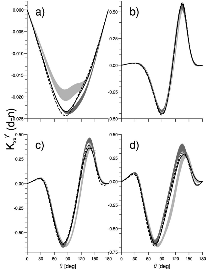
FIG. 9. The spin transfer coefficient K_{xx}^{y'} for elastic Nd scattering. Curves and the sequence of energies as in Fig. 1. pd data at 135 MeV from Ref. [22].
