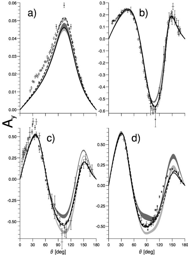
FIG. 2. The analyzing power A_y(N) for elastic Nd scattering. Curves and the sequence of energies as in Fig. 1. Data at 3 MeV from Refs. [61] ( pd crosses) and [54] ( nd circles), at 65 MeV from Refs. [61] ( pd crosses) and [62] ( nd circles), at 135 MeV from Refs. [27] ( pd circles 150 MeV), [64] ( pd crosses 146 MeV), [65] ( pd x's 155 MeV), and at 190 MeV from Refs. [27] ( pd crosses 190 MeV), [66] ( pd circles 198 MeV), [67] ( pd squares 197 MeV).
