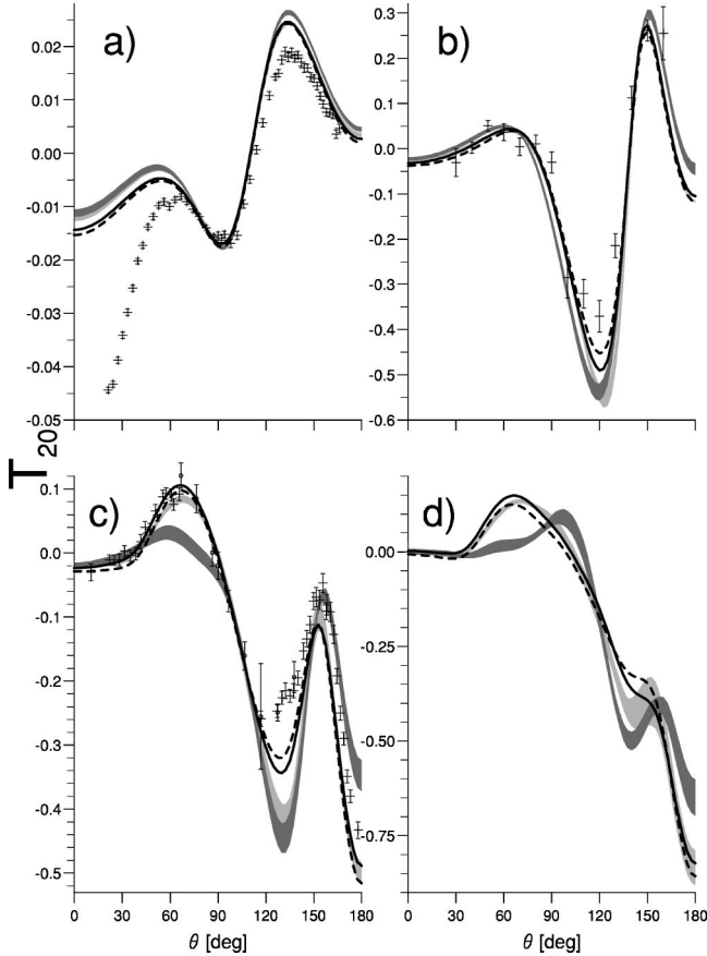
FIG. 4. The tensor analyzing power T_{20} for elastic Nd scattering. Curves and the sequence of energies as in Fig. 1. pd data at 3 MeV from Ref. [61], at 65 MeV from Ref. [68], and at 135 MeV from Refs. [22] (crosses), [23] (circles).
