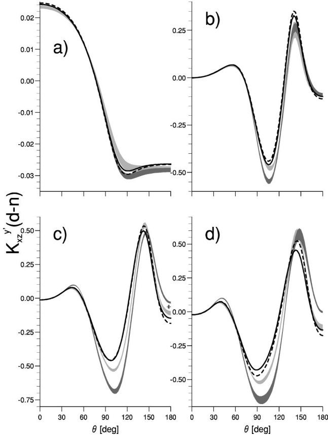
FIG. 10. The spin transfer coefficient K_{xz}^{y'} for elastic Nd scattering. Curves and the sequence of energies as in Fig. 1. pd data at 135 MeV from Ref. [22].
