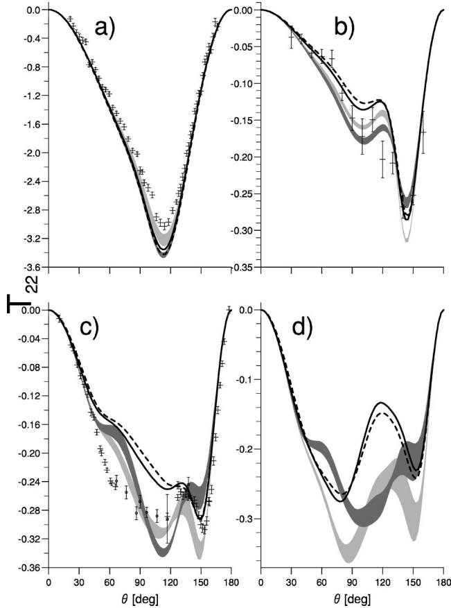
FIG. 6. The tensor analyzing power T_{22} for elastic Nd scattering. Curves and the sequence of energies as in Fig. 1. pd data at 3 MeV from Ref. [61], at 65 MeV from Ref. [68], and at 135 MeV from Refs. [22] (crosses), [23] (circles).
