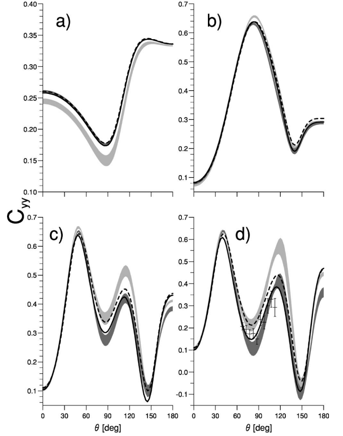
FIG. 13. The spin correlation coefficient C_{yy} for elastic Nd scattering. Curves and the sequence of energies as in Fig. 1. pd data at 190 MeV from Ref. [26].
