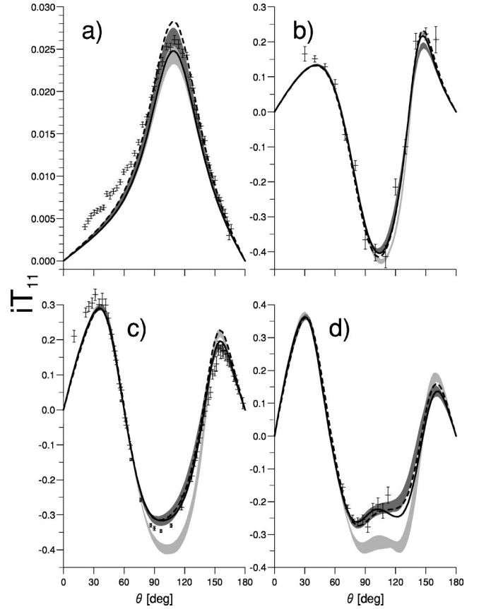
FIG. 3. The deuteron vector analyzing power iT_{11} for elastic Nd scattering. Curves and the sequence of energies as in Fig. 1. pd data at 3 MeV from Ref. [61], at 65 MeV from Ref. [68], at 135 MeV from Refs. [22] (crosses), [23] (circles), and at 190 MeV from [26].
