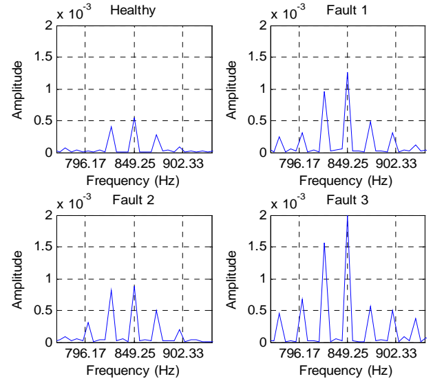
Fig. 7 Spectrum of TSA signals from motor casing for healthy and faulty cases
