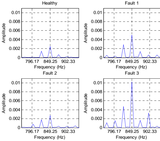
Fig. 6 Spectrum of TSA signals from gearbox casing for healthy and faulty cases
