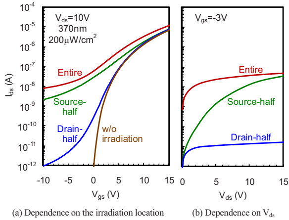
FIG. 2. (Color online) Dependences of I_{\text{leak}} on the irradiation location and V_{\text{ds}} measured using actual ZnO TFTs.
