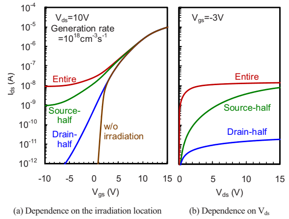
FIG. 3. (Color online) Dependences of I_{\text{leak}} on the irradiation location and V_{\text{ds}} simulated using a 2D device simulation.
