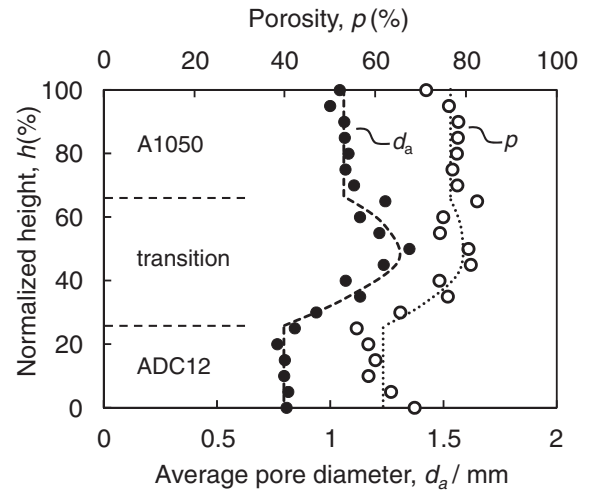
Fig. 3 Relationship between height in the specimen, and porosity and average pore diameter.
