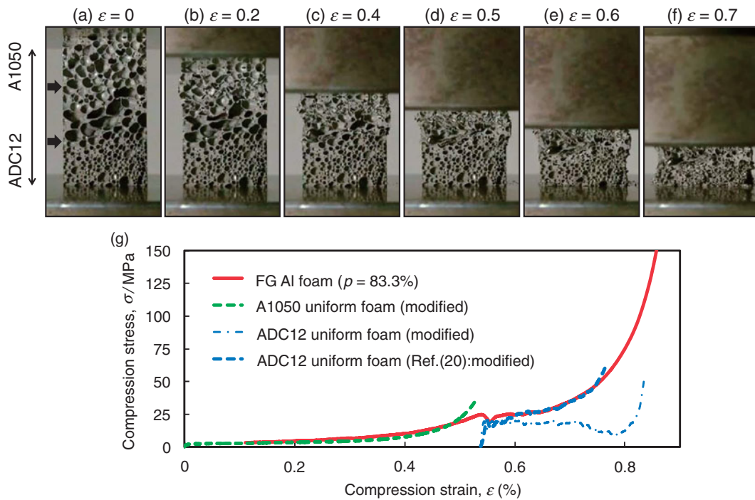
Fig. 4 (a)–(f) Sequential deformation images of FG foam and (g) stress–strain curve of FG foam along with those of uniform A1050 and ADC12 foams.
