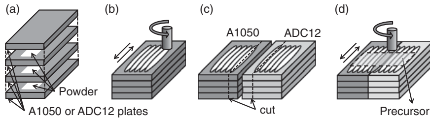
Fig. 1 Schematic illustration of the fabrication process of an A1050–ADC12 FG foam precursor.
