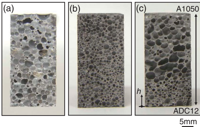
Fig. 2 Compression test specimens of (a) uniform A1050 foam ( p = 87.3\% ), (b) uniform ADC12 foam ( p = 77.4\% ) and (c) A1050-ADC12 FG foam ( p = 83.3\% ).
