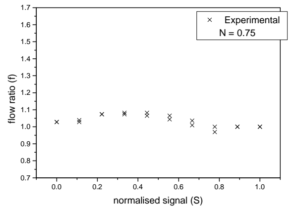
Fig.7 : 50mm valve, initial results
