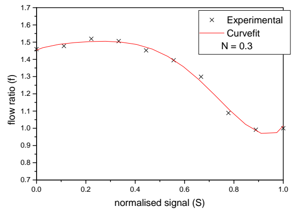
Fig.19 : 50mm valve, downstroke
