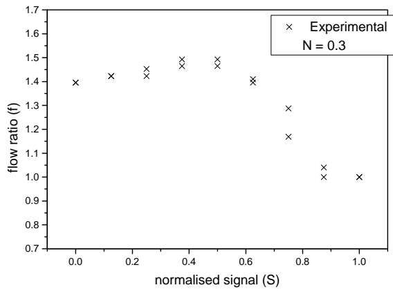
Fig.2 : 40mm valve, initial results
