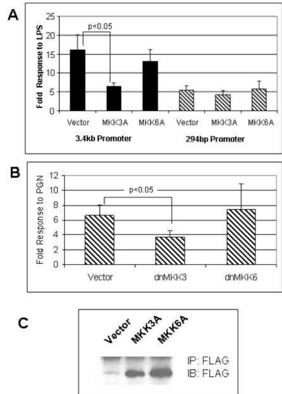
FIG. 7. LPS and PGN induce sIL-1Ra promoter activity via MKK3. RAW 264.7 cells were transiently transfected with sIL-1Ra promoter/luciferase reporters and expression vectors for dominant negative MKK3, MKK6, or empty vector. Cultures were stimulated with 1 \mu g/ml LPS or 10 \mu g/ml PGN for 8 h prior to assay for luciferase activity. Results are means \pm S.D. of three separate experiments. p values were determined by paired t test. A , LPS response. Cells were transfected with either the 3400- or 294-bp IL-1Ra promoters. B , PGN response. Cells were transfected with the 294-bp IL-1Ra promoter reporter. C , immunoblot of whole cell lysates from transfected cells demonstrating the expression of the FLAG-tagged dominant negative MKK proteins as described under “Experimental Procedures.”
