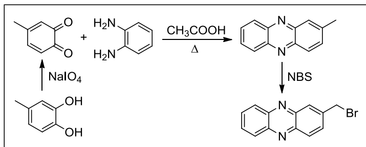
Scheme 2. Preparation of 2-bromomethylphenazine. Reagents and conditions: NaIO 4 , H 2 O, r.t.; CH 3 COOH, reflux, 4 h, 24% (2 steps); NBS, benzoyl peroxide, CCl 4 , reflux, 72 h, 53%.
