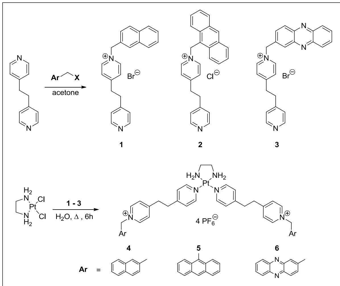
Scheme 1. Target compounds ( 1-6 ). Reagents and conditions: 1,2-bis(4-pyridyl)ethane, \text{ArCH}_2\text{X} , r.t., 24 h, acetone, 74-78%; \text{PtCl}_2(\text{en})_2 , water, reflux, 6 h, 22-61%.
