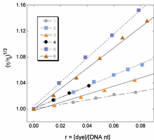
Figure 1. Viscometric measurement experiments of calf thymus DNA and compounds 1-6 at 25 °C (10 mM sodium phosphate buffer, pH = 7.2). Assays were performed at least in duplicate. The averaged slopes are: (1) 0.31 \pm 0.04 , (2) 0.84 \pm 0.03 , (3) 0.65 \pm 0.02 , (4) 0.88 \pm 0.06 , (5) 1.85 \pm 0.11 and (6) 1.59 \pm 0.02 .
